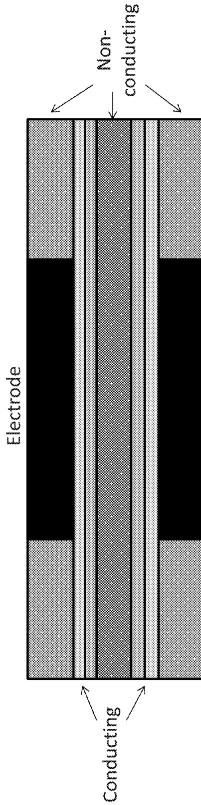
FIG. 12C Double-sided Sensor
